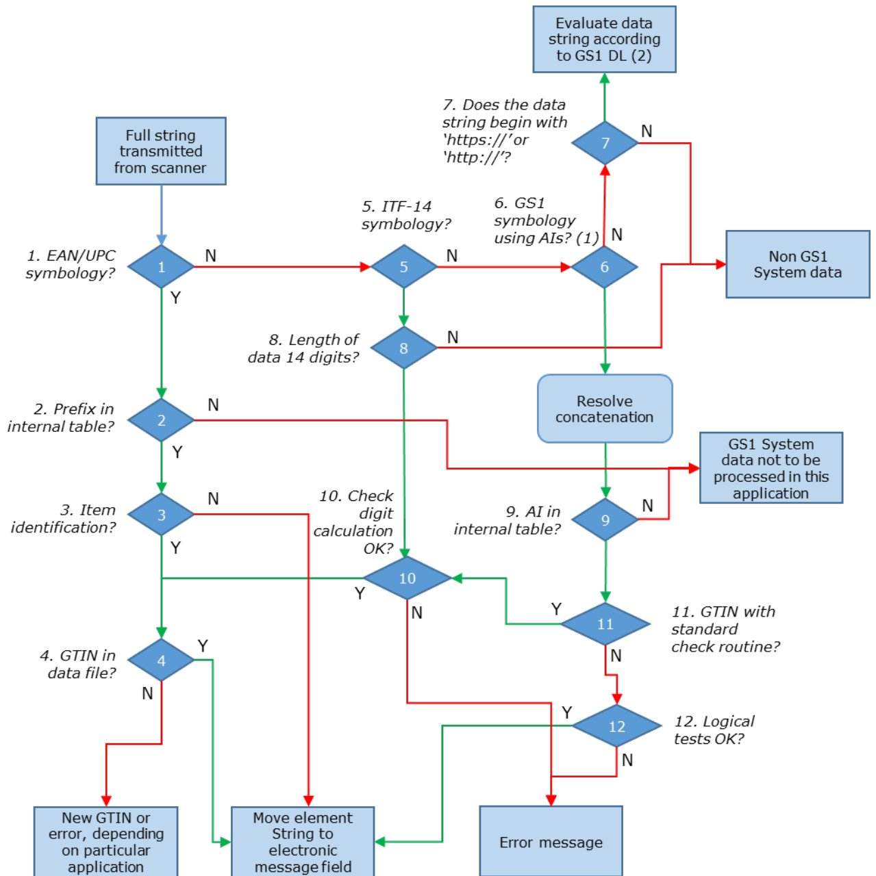
Figure 7.2.1-1. Test procedure
