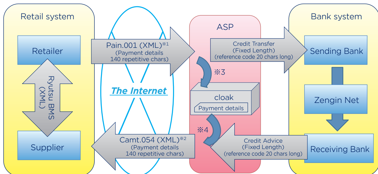
Fig. 2.3-1 Using “cloak” to communicate trade information between retailers and suppliers using ISO20022 messages
